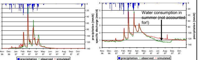
Simulated and observed discharge at the gauges Saer (left) and Yoseph Bridge (right)
